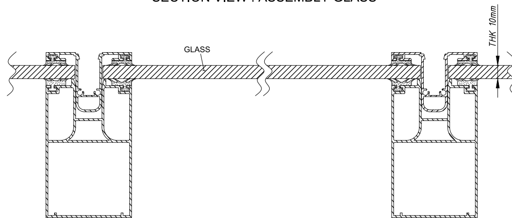
SECTION VIEW : ASSEMBLY GLASS
